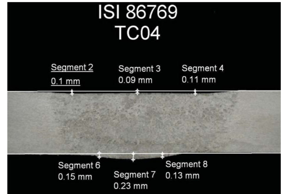
Figure 9: Macrography at 12h.
