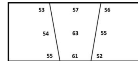
Figure 7: Ferrite content ASTM E562 at 12h.
