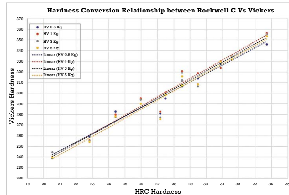
Figure 3. Hardness conversion relation between Rockwell C versus Vickers
