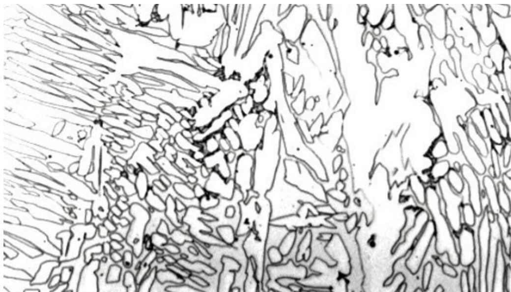
Figure 2. Duplex microstructure with black spots of precipitated intermetallic phases.
