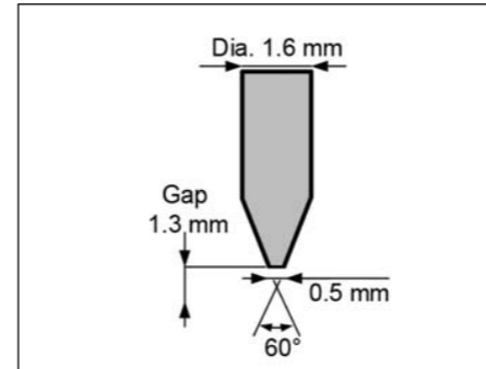
Figure 6: Tungsten electrode preparation.
