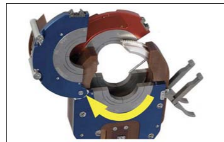
Figure 2: MW40 Polysoude.
