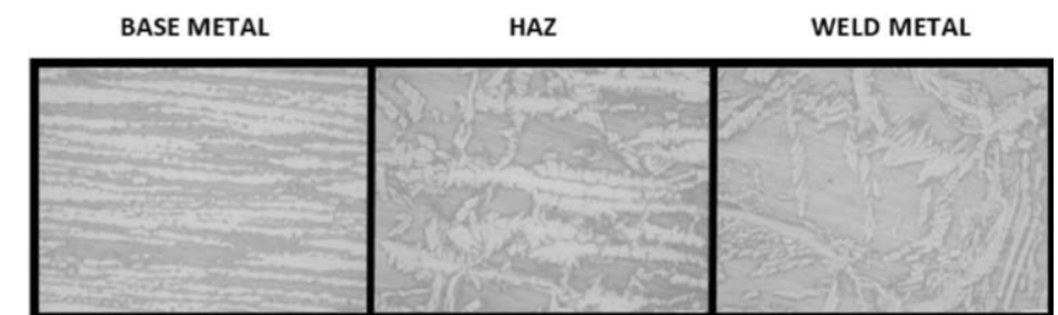
Figure 10: Micrography of base metal, HAZ, weld metal at 12h.
