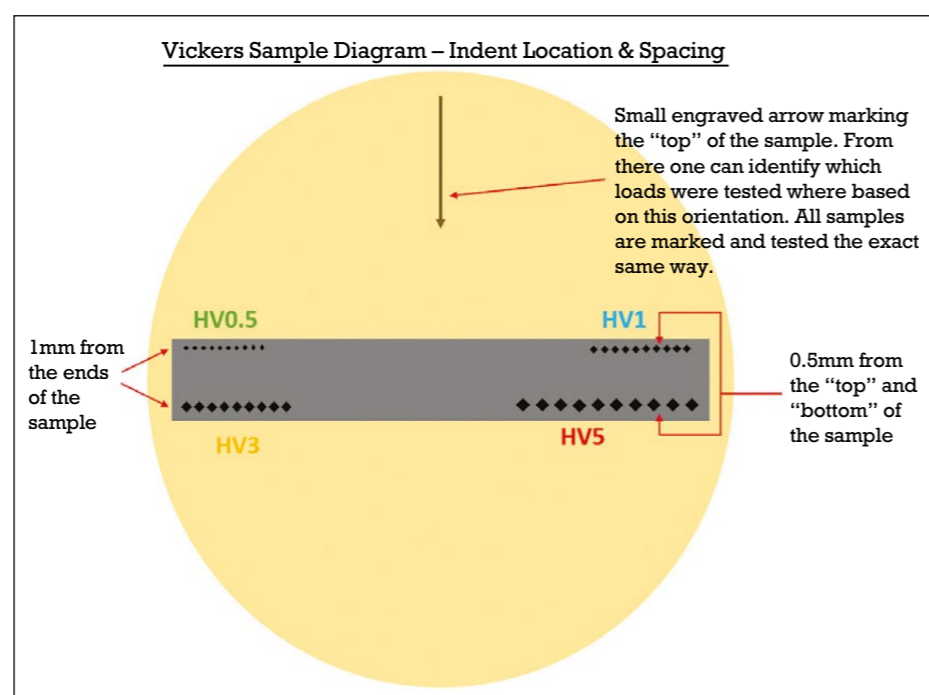
Figure 1. Vickers micro-hardness location
