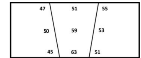
Figure 8: Ferrite content ASTM E562 at 6h.
