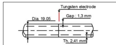
Figure 4: Welding preparation.
