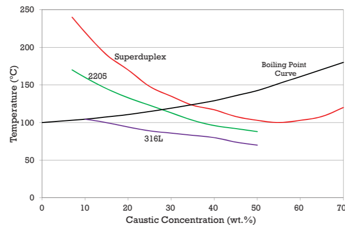
Figure 2. Iso-corrosion curves (0.1 mm/y) for some stainless steels in caustic soda 3 .
