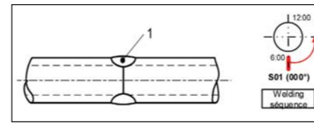
Figure 5: Welding sequence.
