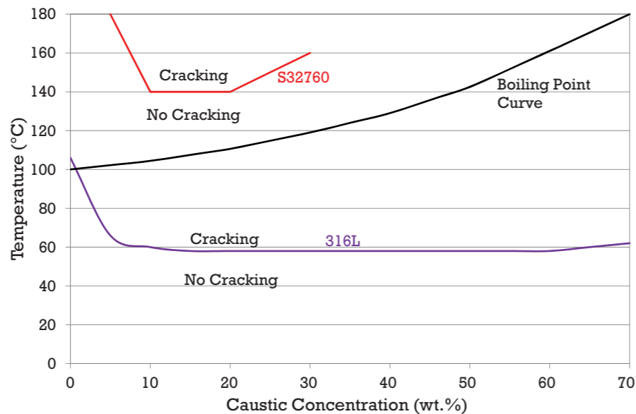
Figure 7. Conservative SCC limits for 316L and S32760 superduplex under strongly oxidizing conditions 3, 5 .
