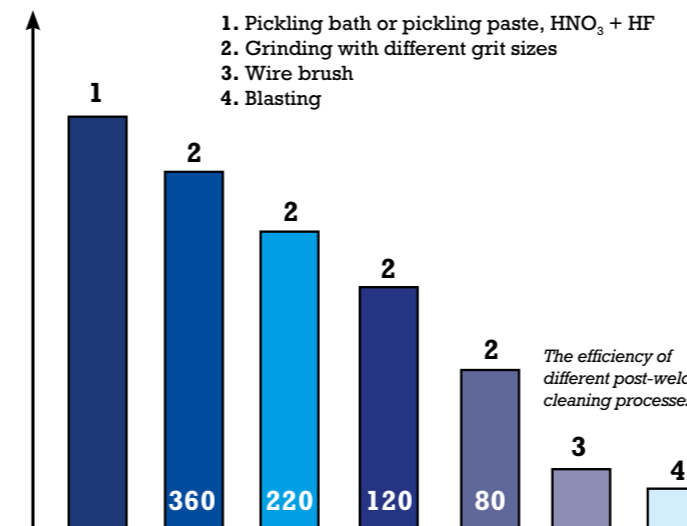
Figure 3. The efficiency of different post weld cleaning processes on the pitting potential.
