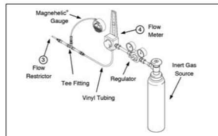
Figure 3: SWS internal purge pressure kit Swagelok.
